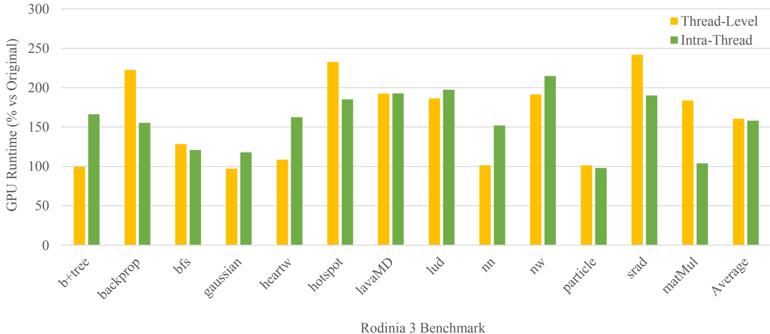
Thread-Level vs Intra-Thread Duplication (Titan Xp)
