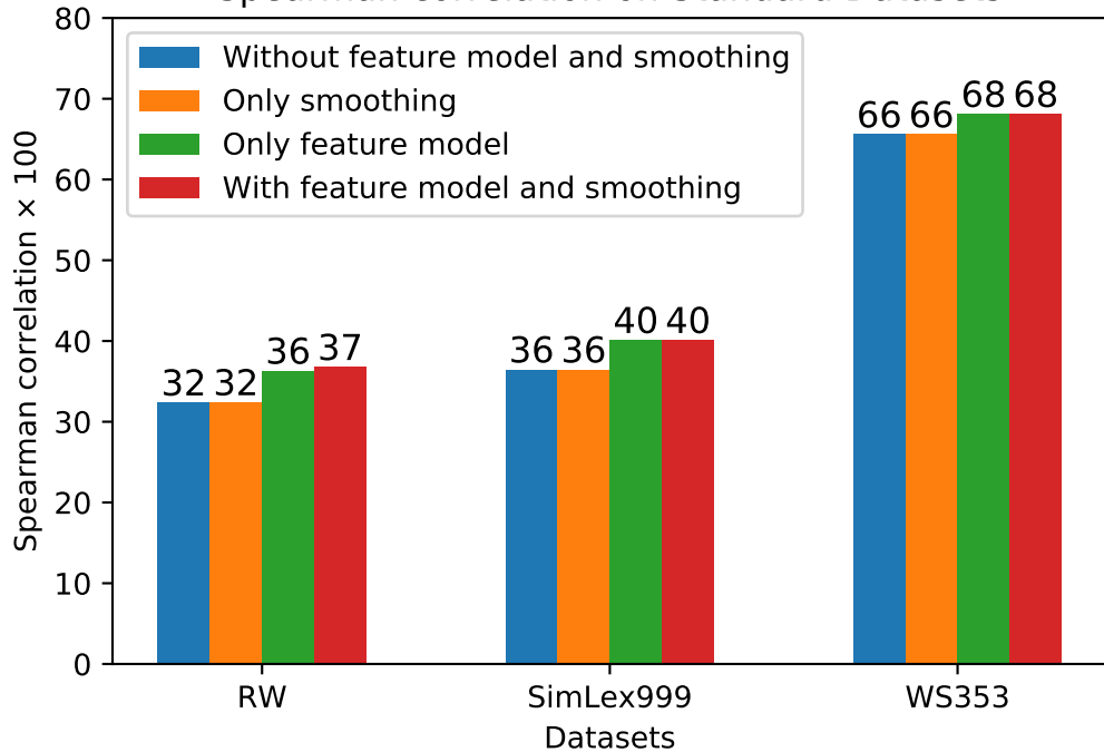
Spearman correlation on Standard Datasets
