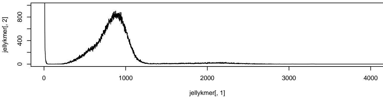
Jellyfish k=23
